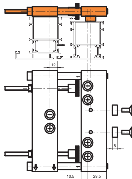
Nodo laterale R60TT R60TT side section Articulación lateral R60TT
